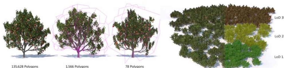
Fig. 4: Left side: Full polygonal tree model and two simplified versions each with an upper limit for the polygon count generated with our system. Right side: Visualization of a large botanical scene. Color indicates different levels of detail.
